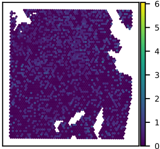
SNU51A RNF103 expression Moran's I = 0.01
