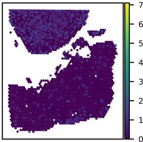
SNU25A ANKRD34A expression Moran's I = 0.23
