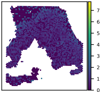
SNU18A POLR3D expression Moran's I = 0.12
