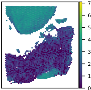
SNU25A SNAP25 expression Moran's I = 0.85
