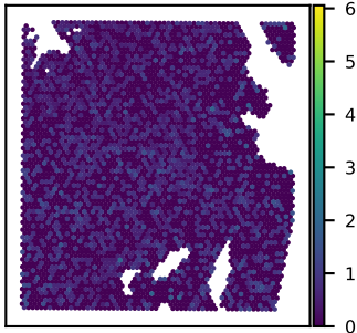
SNU51A ZFP30 expression Moran's I = 0.01
