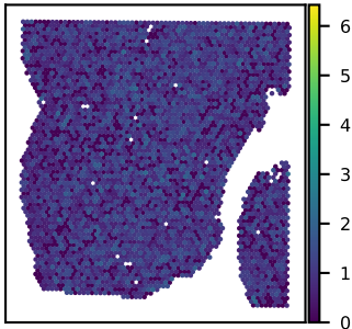
SNU25B SLC30A9 expression Moran's I = 0.03
