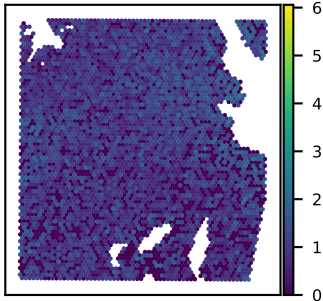
SNU51A CHMP3 expression Moran's I = 0.07
