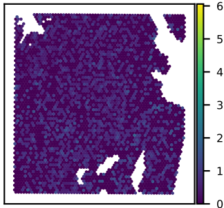
SNU51A SLC66A1 expression Moran's I = 0.02
