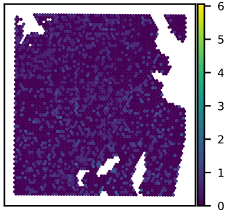
SNU51A BANP expression Moran's I = 0.03
