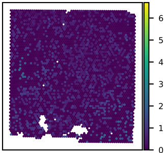
SNU43A MTHFD2L expression Moran's I = 0.02
