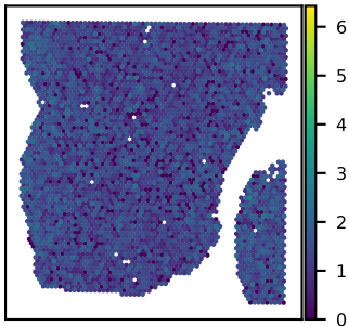
SNU25B HNRNPH1 expression Moran's I = 0.04
