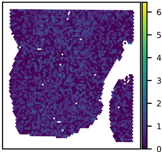
SNU25B CNTNAP2 expression Moran's I = 0.06
