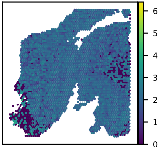
SNU24A NDUFS5 expression Moran's I = 0.17
