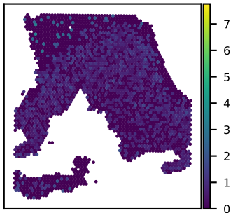
SNU18A SLC7A8 expression Moran's I = 0.08
