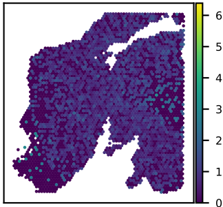
SNU24A BTN3A3 expression Moran's I = 0.06
