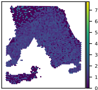
SNU18A NCSTN expression Moran's I = 0.18
