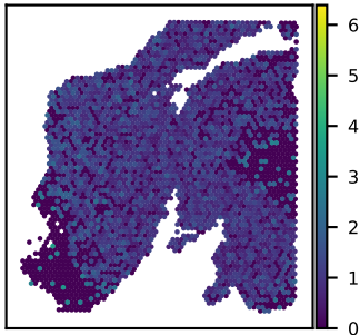
SNU24A PAQR4 expression Moran's I = 0.10
