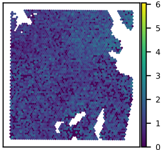
SNU51A STMN4 expression Moran's I = 0.12
