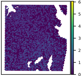
SNU51A PLXNA3 expression Moran's I = 0.03
