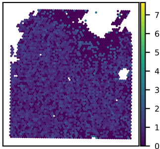
SNU21B PANK3 expression Moran's I = 0.08
