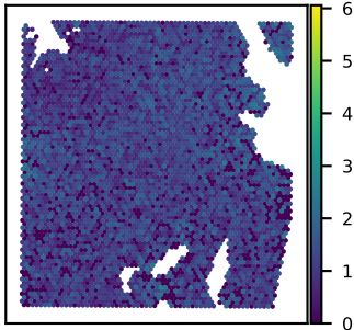
SNU51A NPDC1 expression Moran's I = 0.05
