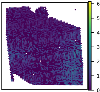
SNU27A CAMK2G expression Moran's I = 0.22
