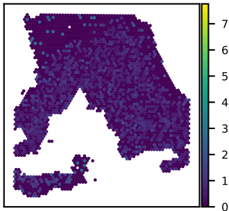
SNU18A CLEC16A expression Moran's I = 0.05
