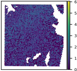
SNU51A RNF13 expression Moran's I = 0.09
