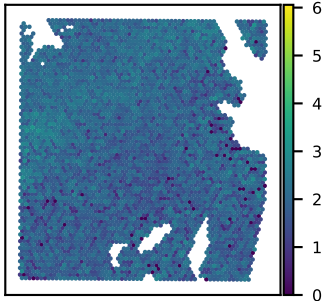
SNU51A TMBIM6 expression Moran's I = 0.15
