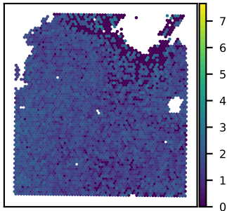
SNU21B TMEM165 expression Moran's I = 0.16
