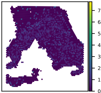
SNU18A UBASH3B expression Moran's I = 0.09
