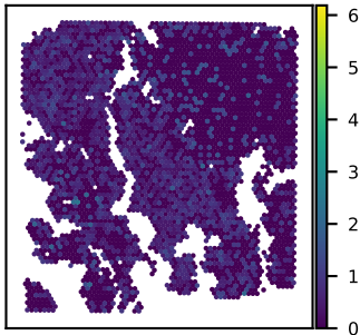
SNU16B LMNB1 expression Moran's I = 0.08
