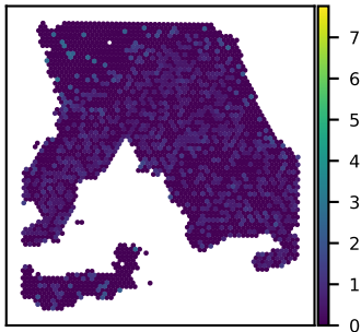
SNU18A ZNF263 expression Moran's I = 0.02
