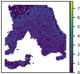
SNU18A CSGALNACT2 expression Moran's I = 0.11
