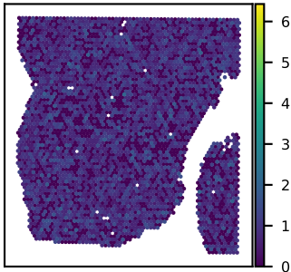
SNU25B SLC25A28 expression Moran's I = 0.02
