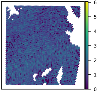
SNU51A MAP2K2 expression Moran's I = 0.08
