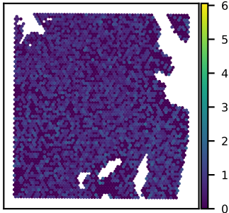
SNU51A EHMT1 expression Moran's I = 0.02
