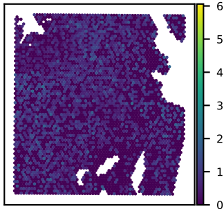
SNU51A SLC38A3 expression Moran's I = 0.05
