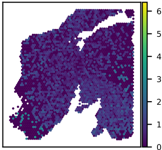
SNU24A ARHGAP11A expression Moran's I = 0.13
