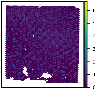
SNU43A SLC35E2A expression Moran's I = 0.02
