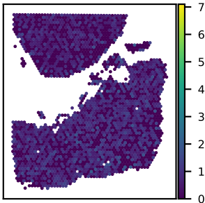
SNU25A SMARCD2 expression Moran's I = 0.03
