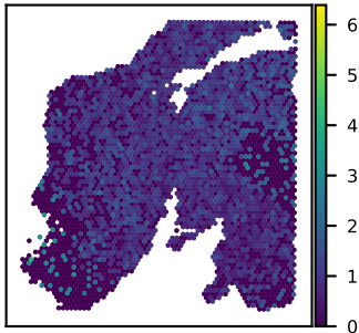
SNU24A PECAM1 expression Moran's I = 0.09
