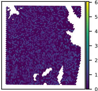
SNU51A PRMT7 expression Moran's I = 0.01
