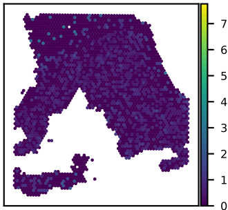
SNU18A ZNF568 expression Moran's I = 0.01
