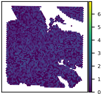
SNU24B TMEM170A expression Moran's I = 0.04
