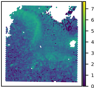
SNU21B COL4A1 expression Moran's I = 0.65
