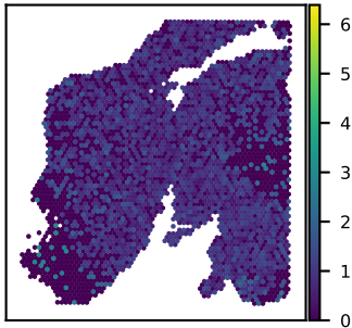
SNU24A DNTTIP2 expression Moran's I = 0.05
