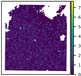
SNU21B SREK1IP1 expression Moran's I = 0.05
