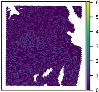
SNU51A GCNT2 expression Moran's I = 0.02
