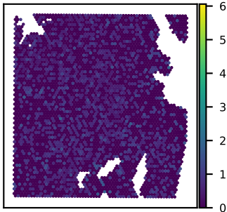
SNU51A PYM1 expression Moran's I = 0.00
