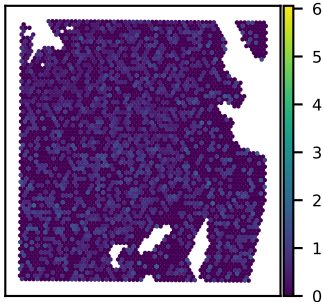
SNU51A TMEM216 expression Moran's I = 0.01
