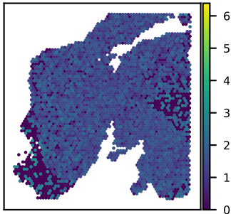
SNU24A PPP6R2 expression Moran's I = 0.10
