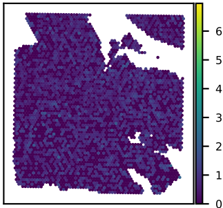
SNU24B SNRNP35 expression Moran's I = 0.01
