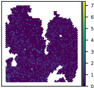
SNU27B CSRNP1 expression Moran's I = 0.05
